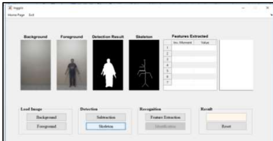
Figure 8 Detection Result (Skeleton)
