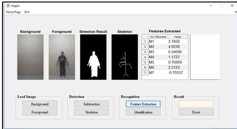
Figure 9 Recognition feature extraction with moment invariant
